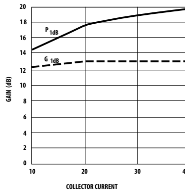
Figure 3. AT-41586 P_{1dB} and G_{1dB} vs. Collector Current at V_{CE} = 8\text{ V} , f = 2.0\text{ GHz} .
